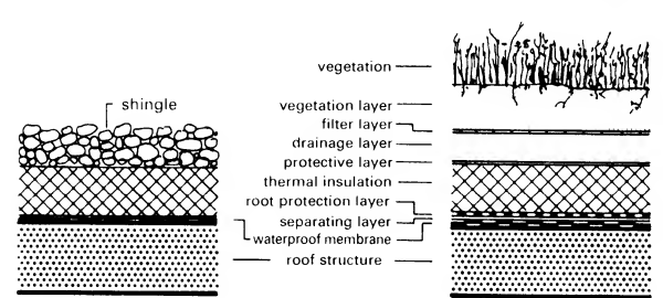
⑤ Inverted roof → ⑥
